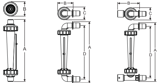
Adjustable Panel Mount
